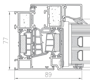
CROSS SECTION THROUGH TM 77EI 30 WINDOW
